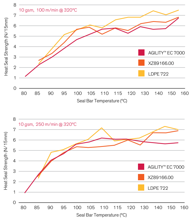
Seal Strength Comparison
